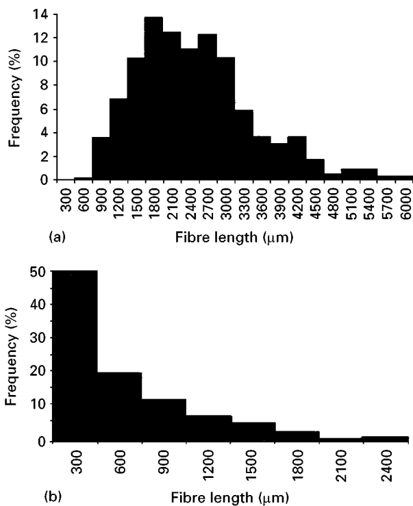
Figure 1 Fibre length distributions for wheat straw, (a) before processing with PP, (b) after solvent extraction from PP.
