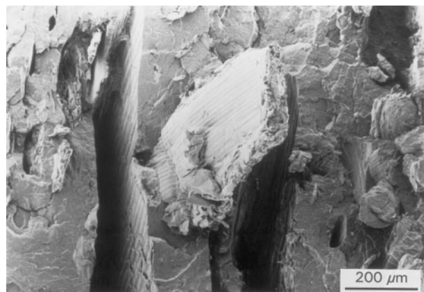
Figure 4 Fracture surface showing lack of adhesion between polypropylene and wheat straw.
