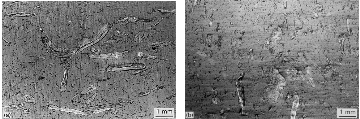
Figure 7 Reflected light micrographs of injection-moulded polypropylene composites containing flax straw fibres: (a) skin region, parallel to the flow direction, and (b) core region, normal to the flow direction.
