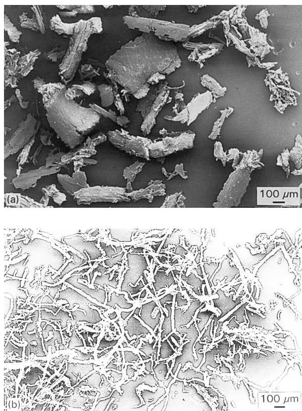
Figure 2 Structure of natural fibres after extraction from moulded polypropylene composites: (a) wheat straw and (b) flax straw.
