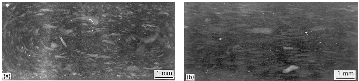
Figure 6 Contact microradiographs of injection-moulded polypropylene containing wheat straw fibres (a) normal to the flow direction and (b) parallel to the flow direction.
