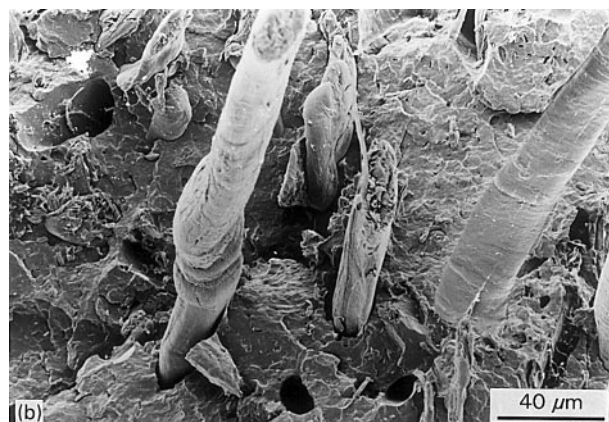
Figure 3 Fracture surfaces of polypropylene composites containing (a) wheat straw and (b) flax straw fibres.
