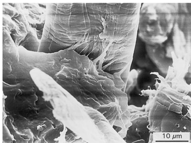
Figure 8 Fibre–matrix bonding in polypropylene/flax straw composite containing MA-PP.
