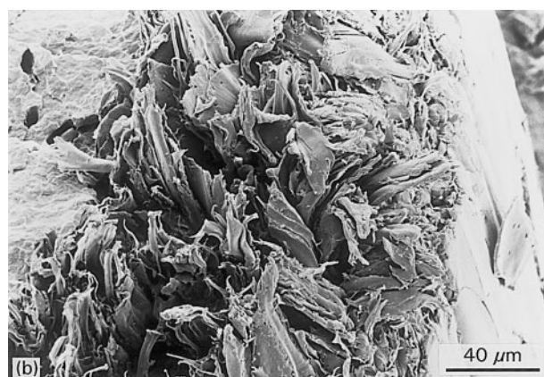
Figure 5 Collapse in cellular structure of wheat straw (a) before and (b) after melt processing with polypropylene.
